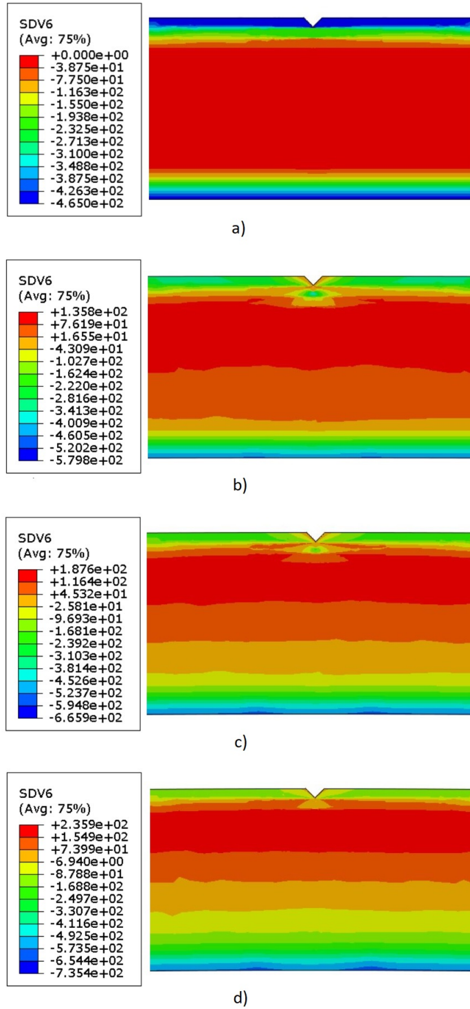
Figure 5.4: Stress evolution with d_{ol}=134\mu m and c_s=465Mpa a) disp=0 , residual stress b) disp=0.1 c) disp=0.2 d) disp=0.3
