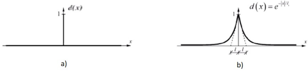
Figure 2.1: 1d bar a)sharp crack b)diffused crack
